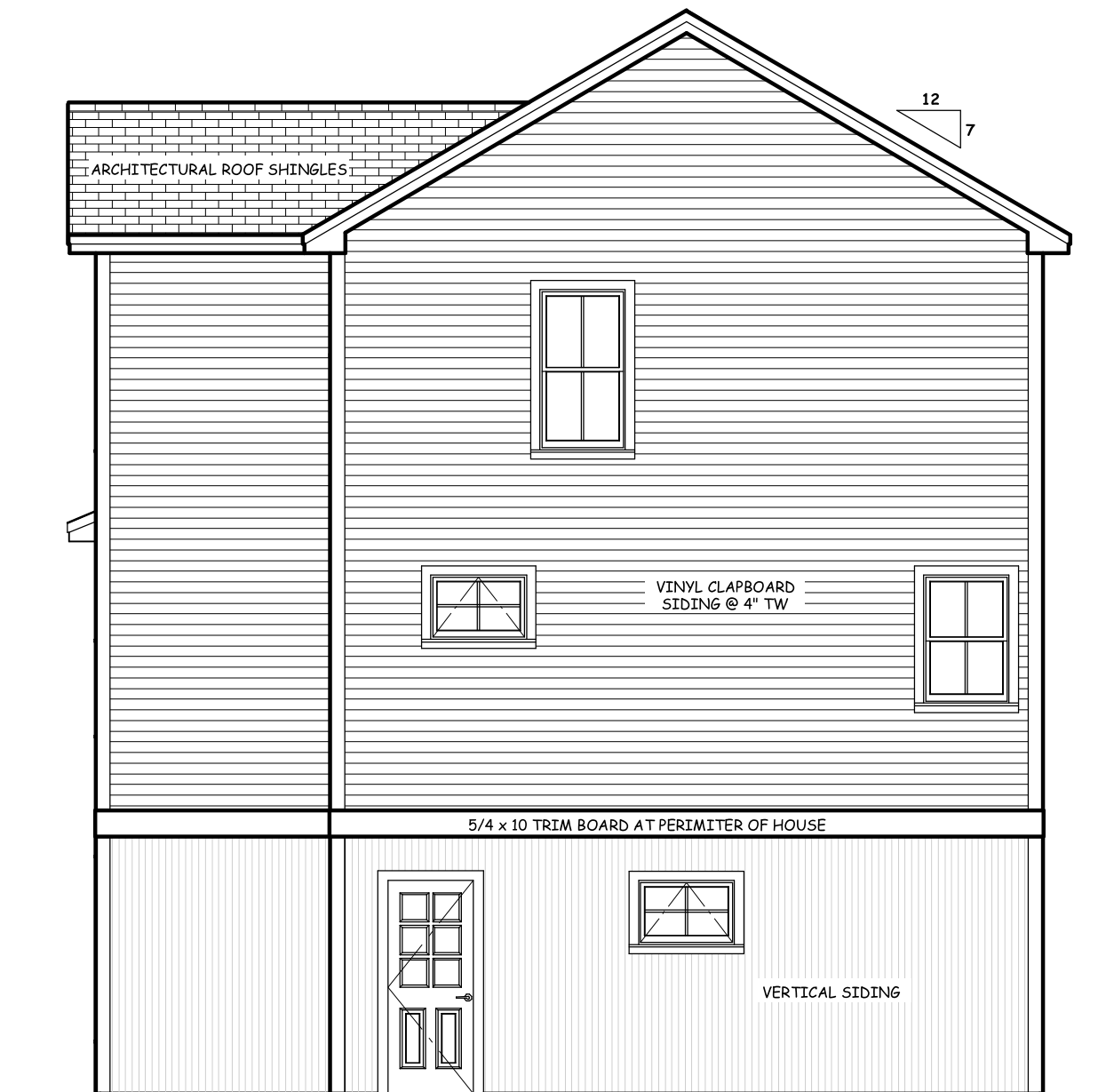
BACK ELEVATION
